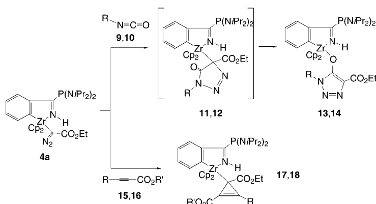
Scheme 3. Cycloaddition reactions of the \alpha -diazomethyl zirconium complex 4a . 9 , 11 , 13 : R = Ph; 10 , 12 , 14 : R = \alpha -Naph; 15 , 17 : R = \text{CO}_2\text{Et} , R' = Et; 16 , 18 : R = H, R' = Me.
